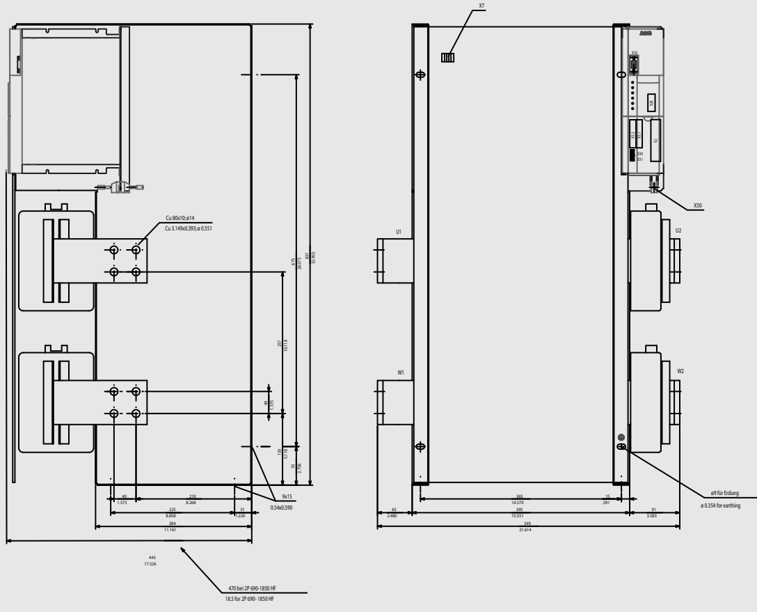
Thyro-P 2P (1850 HF, 2000 HF)
